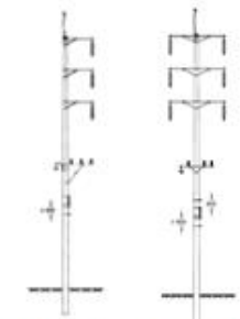
Concrete pole
